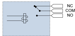
Relay On
