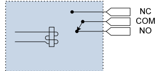
Relay On
