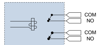
Relay On
