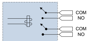
Relay Off
